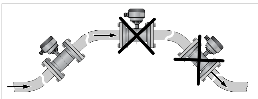
Figure 2-9: Installation in bending pipes (45°)
