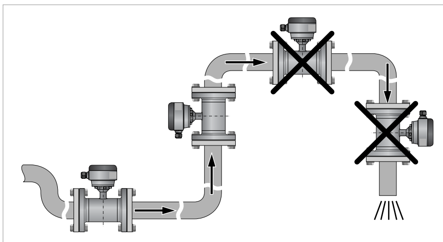
Figure 2-8: Installation in bending pipes (90°)
