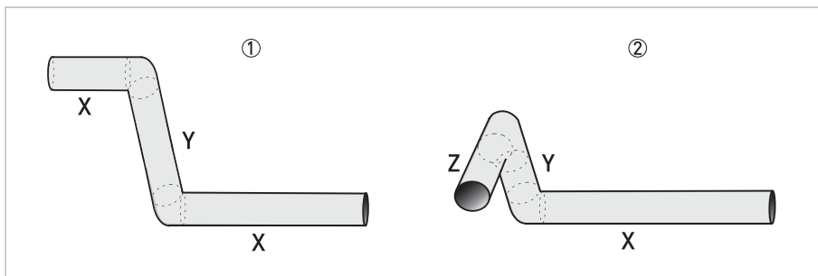
Figure 2-6: 2 and/or 3 dimensional bends upstream of the flowmeter
