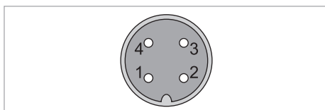
Figure 4-3: M12 quick disconnect plug
