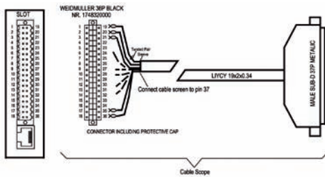
Cable connection diagram
