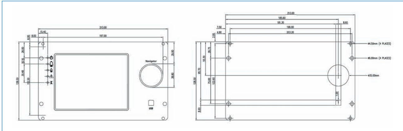
Dimensions [mm]
