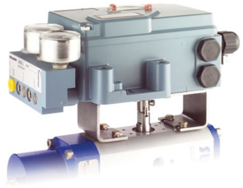
Example for mounting on rotary actuators.
